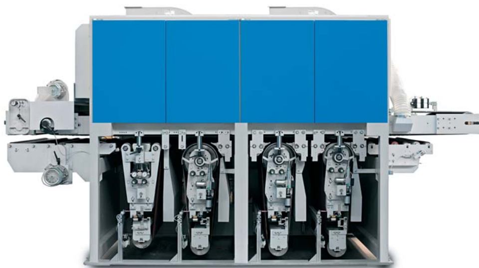
Calibratrice-levigatrice inferiore Bottom calibrating-sanding machine Unten arbeitende Kalibrier-Schleifmaschine
